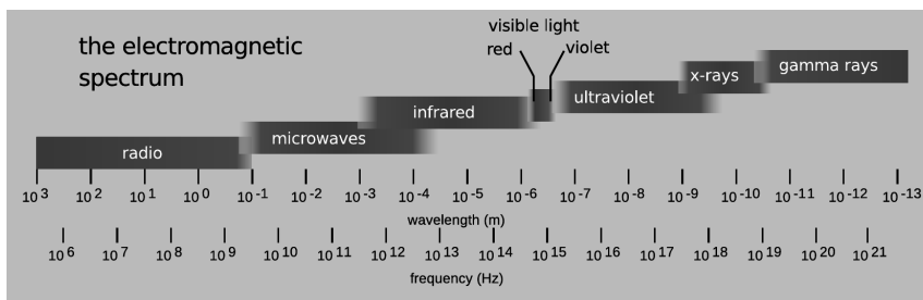
o / The electromagnetic spectrum.
